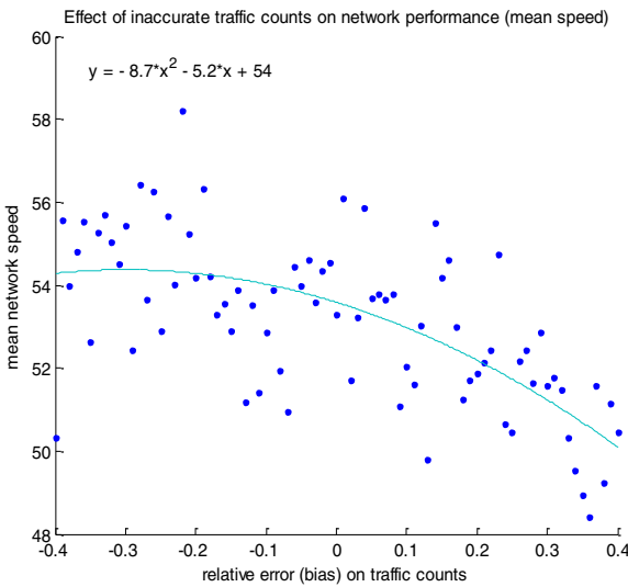
Fig. 4 Effect of a fixed error of the measured traffic counts on the mean network speed ( r^2 = 0.44 ).
